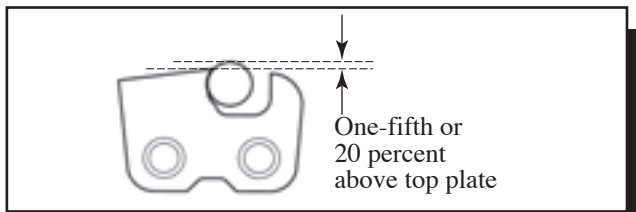
Figure 3-11—Hold the file at least one-fifth of the file’s diameter above the cutter’s top plate.—Oregon Maintenance and Safety Manual, permission by Blount, Inc.
