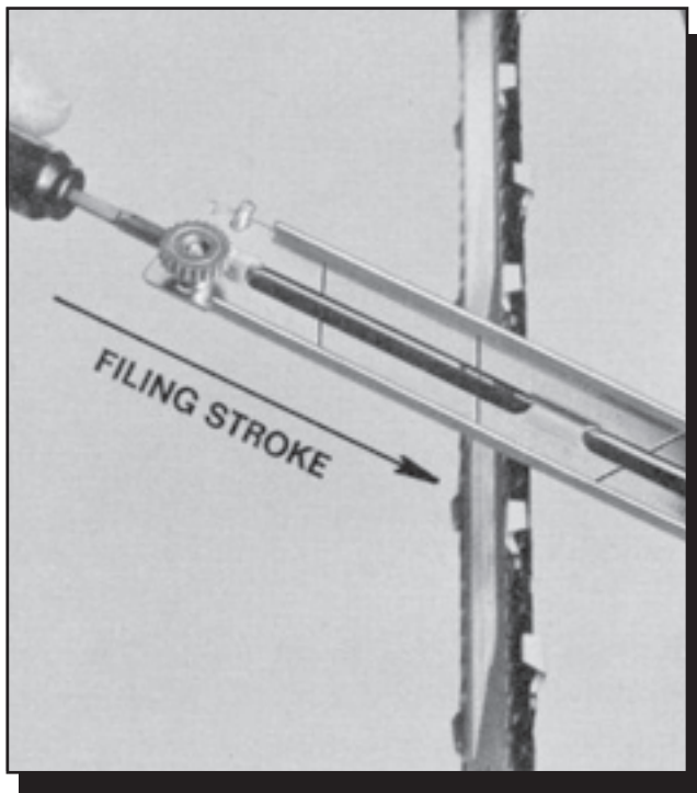
Figure 3-12—The correct top-plate angle is marked on the file guide.—Oregon Maintenance and Safety Manual, permission by Blount, Inc.
